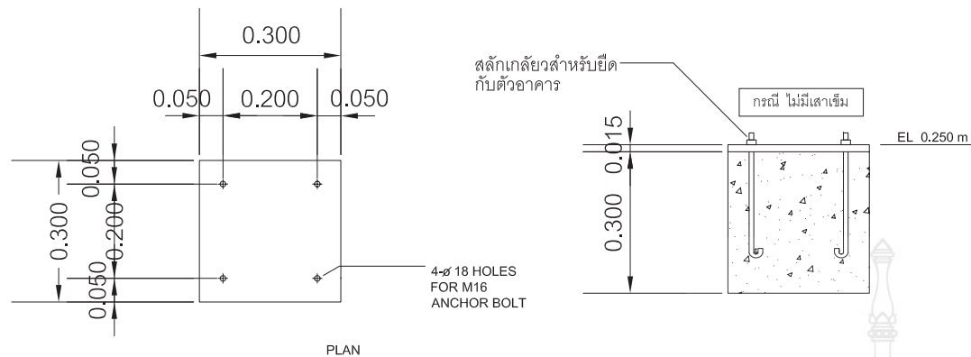
DETAIL FOR F3
