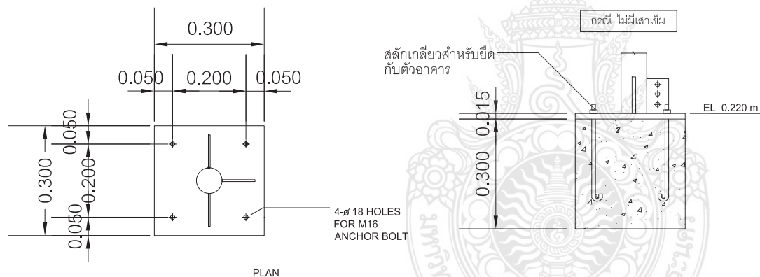
DETAIL FOR F2
